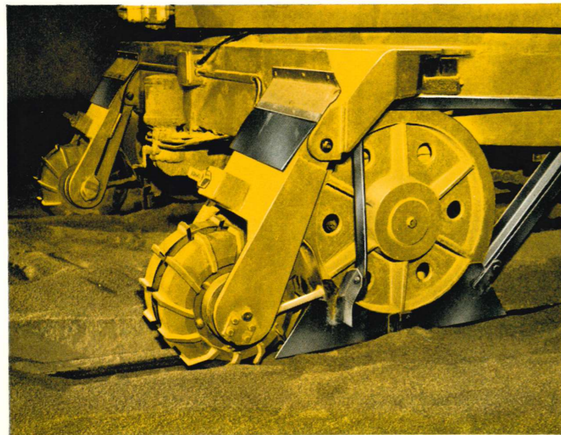
Rail milling material cutters for scraper loader
