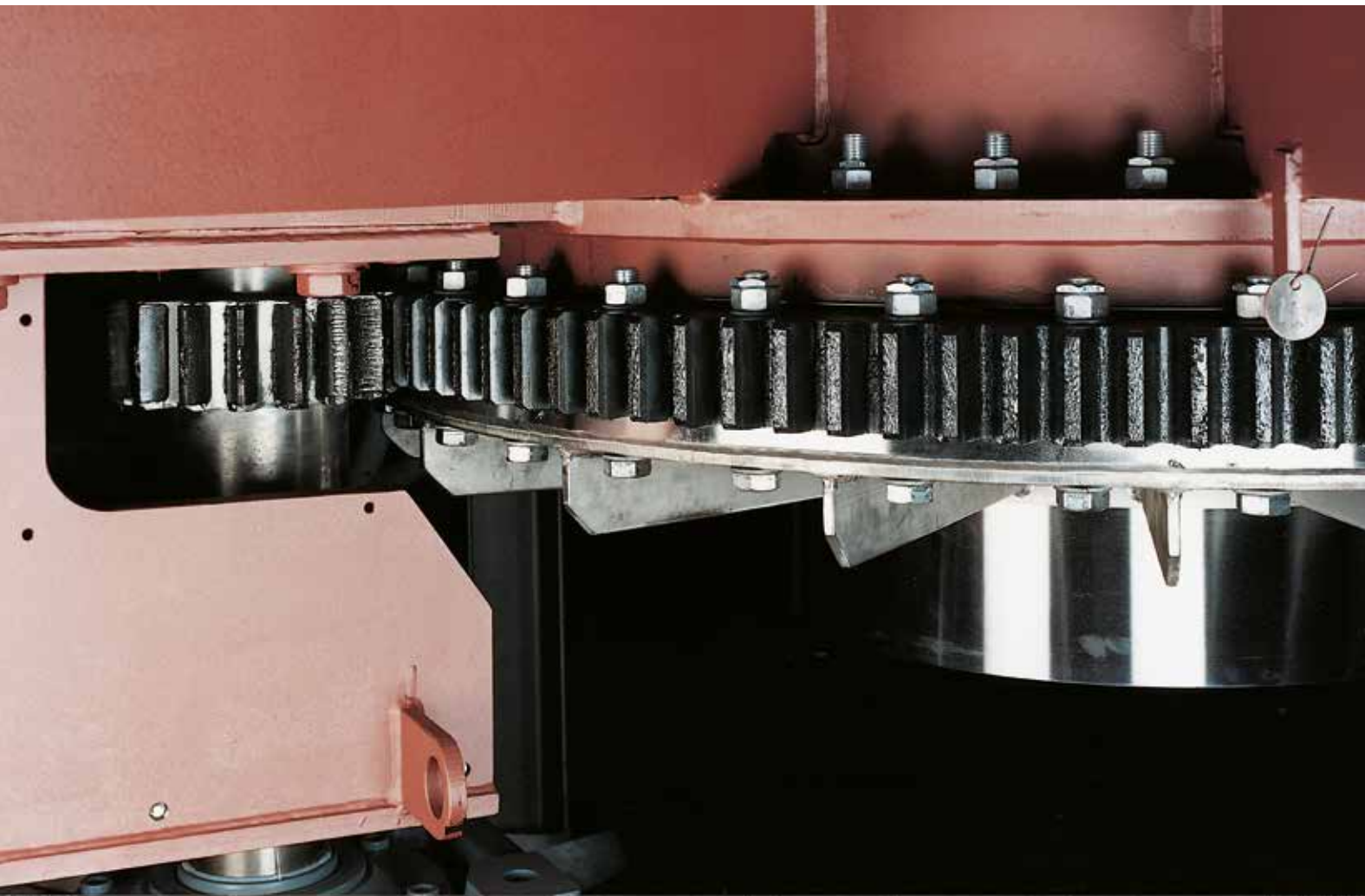
Drive arrangement of CTX-AV, external drive (close up)
