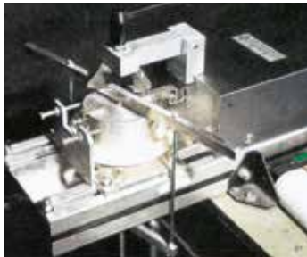
Jennicke shear cell
