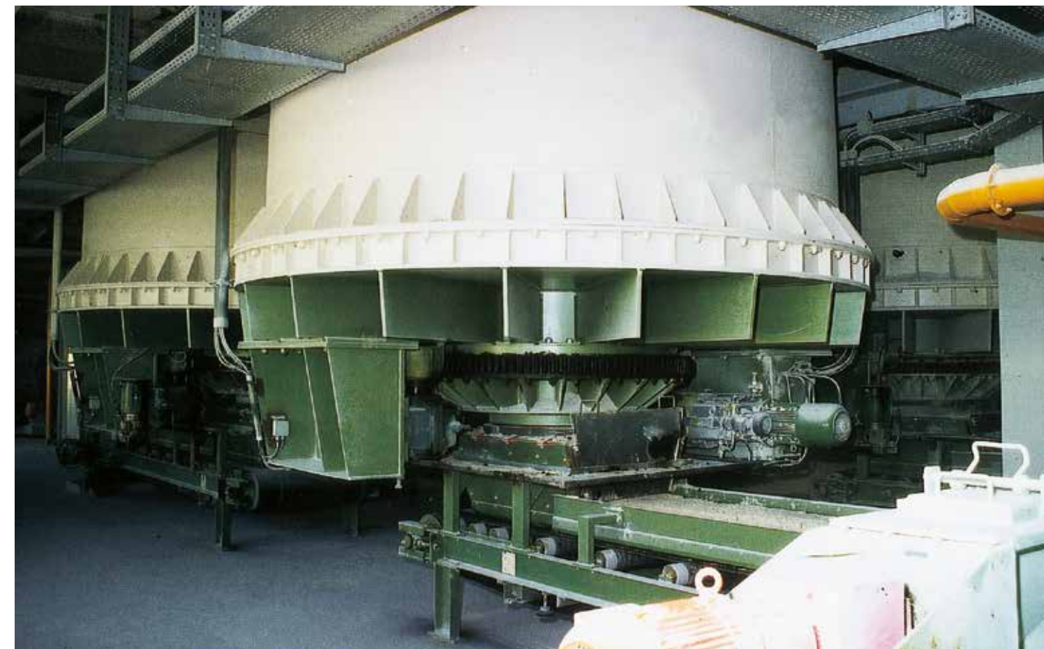
CENTREX® with two external drives for discharge of FGD Gypsum loading onto a weigh feeder
