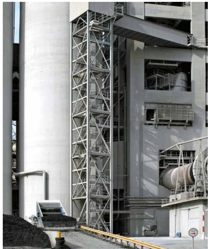
Regulated discharge with screw metering feeder direct to bucket elevator
