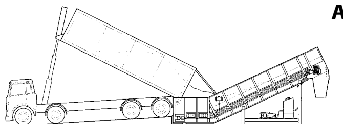
Material is drawn into the empty Samson® MF body by the forward moving apron-belt
