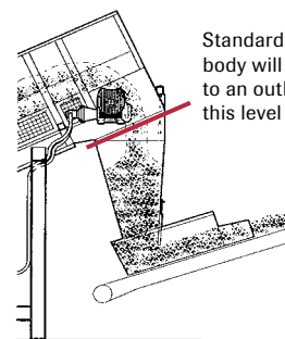
Centralising head chute
